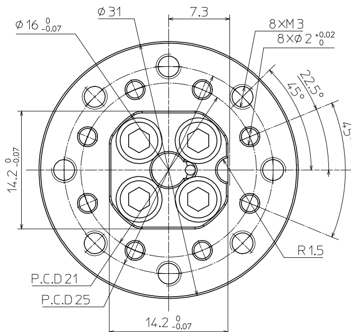
Servo Horn
