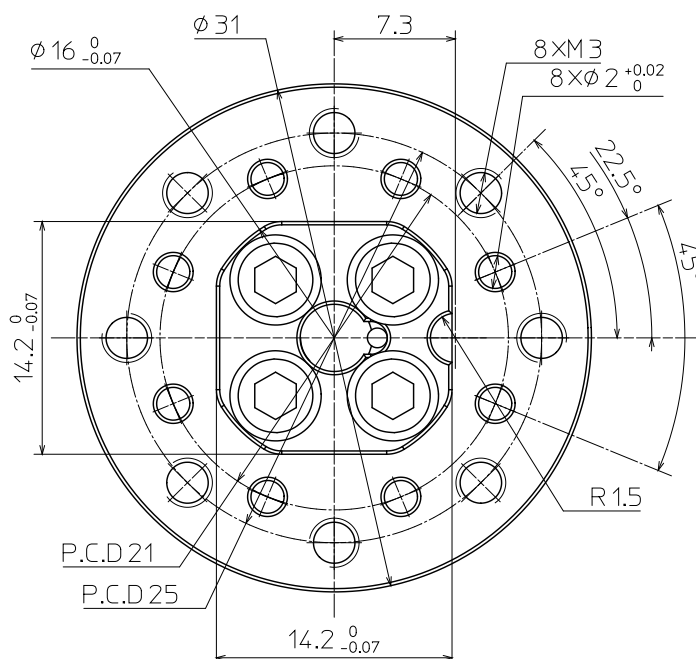
Servo Horn
