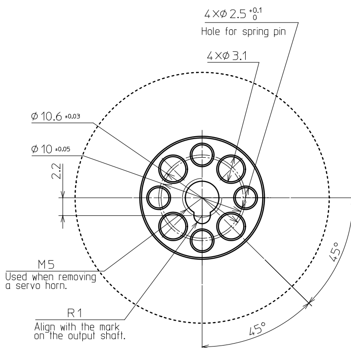
Mounting point for a servo horn
