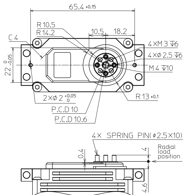
Without Servo Horn
